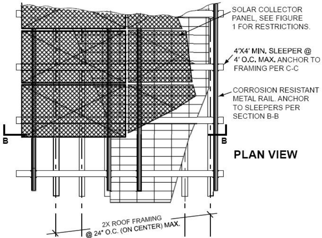
Figure 305.3.3.1.1(2) Installation – Rails parallel to framing members
